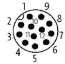
M12 Male
